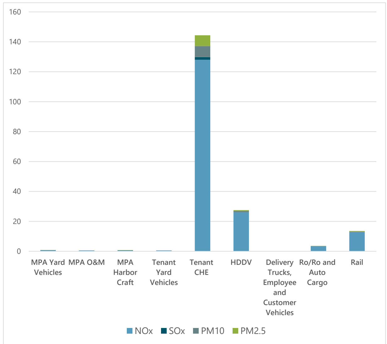
Figure 2 2020 CAP Mobile Source Emissions (tons/year)
