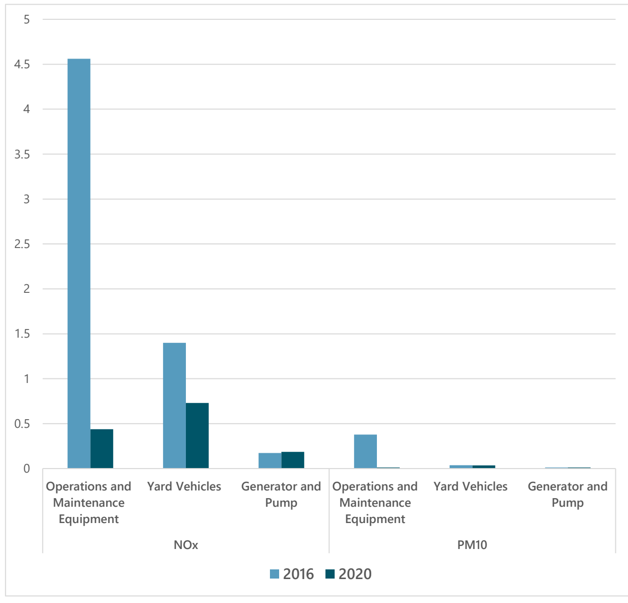
Figure 5 MPA Engine Based NO x and PM 10 Emissions (tons/year) 2016 vs 2020
